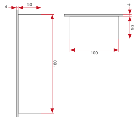
Rear section of casing
