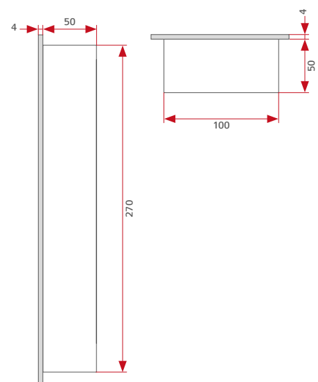
Rear section of casing
